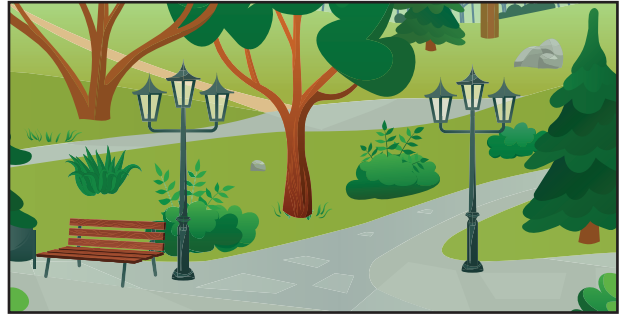
a park
