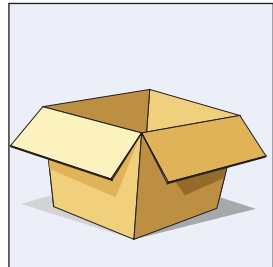
box
