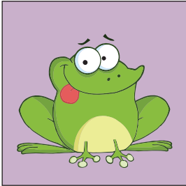
frog
