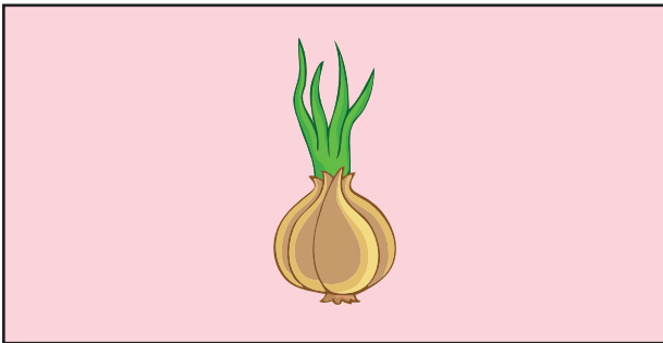
an onion
