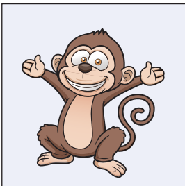
monkey
