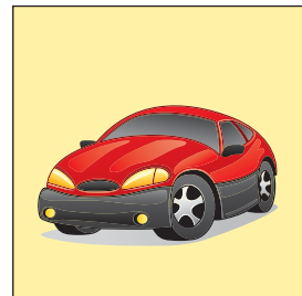
car
