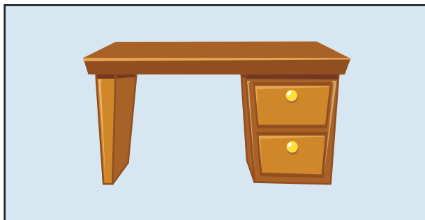
a desk
